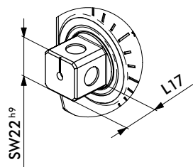
Dimensions of the driven shaft
