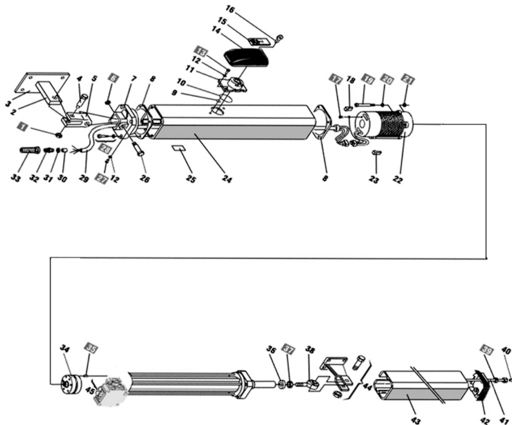
Exploded sight
